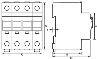
Dimensional drawing Group view
