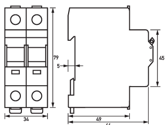
Dimensioned drawing switch-disconnectors RH 040-200
