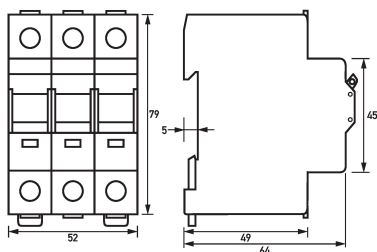
Dimensioned drawing switch-disconnectors RH
