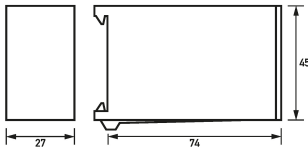
Dimensioned drawing mounting tools Coron Do1 HF
