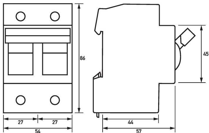
Dimensional drawing Coron 2 (Group view)
