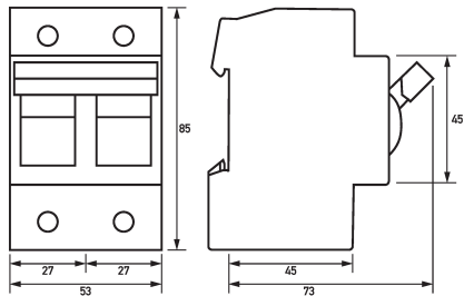
Dimensioned drawing fuse-switch-disconnector Coron 2 Do-63-2
