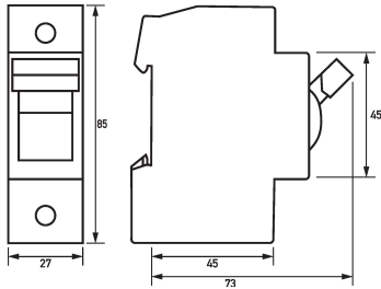
Dimensioned drawing fuse-switch-disconnector Coron 2 Do-63-1
