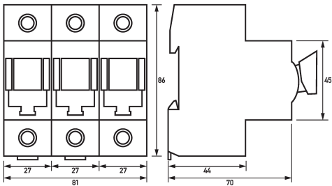
Dimensioned drawing fuse-switch-disconnector Tytan
