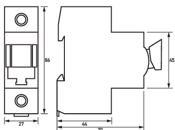
Dimensioned drawing fuse-switch-disconnector Tytan
