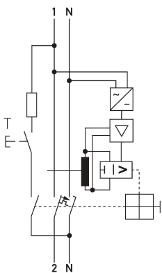
Wiring example residual current operated circuit-breakers with integral overcurrent protection DRCBO 4 C25/0,10/1N-HP
