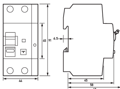
Dimensioned drawing residual current operated circuit-breakers with integral overcurrent protection DRCBO 4 C25/0,10/1N-HP
