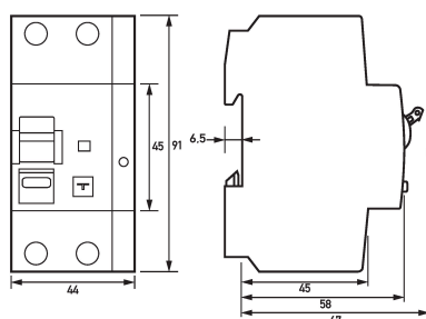
Dimensioned drawing residual current operated circuit-breakers with integral overcurrent protection DRCBO 4 B13/0,30/1N-B+
