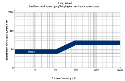
Characteristic B NK 100 mA
