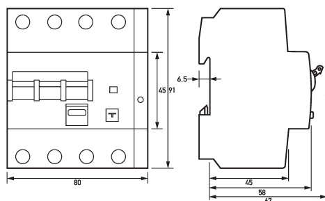
Dimensioned drawing residual current operated circuit-breakers with integral overcurrent protection DRCBO 4 C32/0,03/3N-B+
