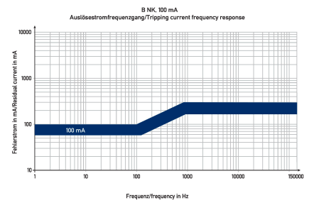
Characteristic B NK 100 mA
