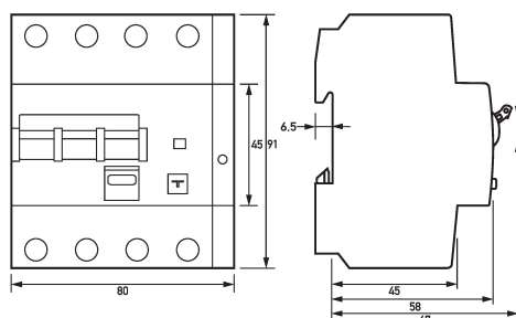
Dimensioned drawing residual current operated circuit-breakers with integral overcurrent protection DRCBO 4 C32/0,10/3N-B SK
