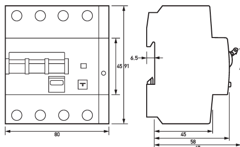
Dimensioned drawing residual current operated circuit-breakers with integral overcurrent protection DRCBO 4 C13/0,10/3N-B SK
