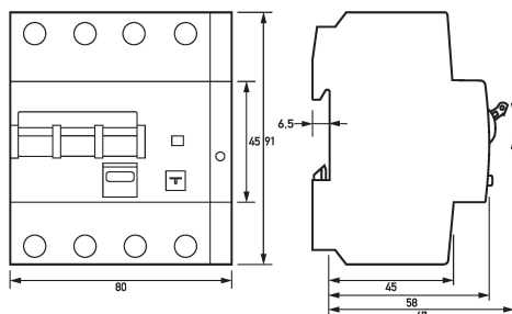
Dimensioned drawing residual current operated circuit-breakers with integral overcurrent protection DRCBO 4 C13/0,03/3N-B SK
