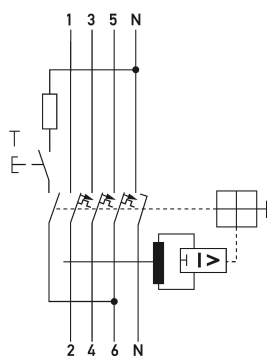
Wiring example residual current operated circuit-breakers with integral overcurrent protection DRCBO 4 B20/0,03/3N-A
