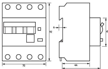
Dimensioned drawing residual current operated circuit-breakers with integral overcurrent protection DRCBO 4 B20/0,03/3N-A
