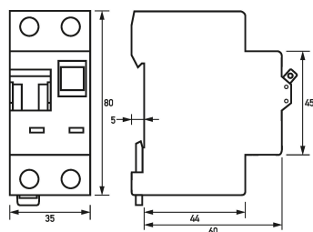
Dimensioned drawing residual current operated circuit-breakers with integral overcurrent protection DRCBO 3 Type AC, C-characteristic, 1+N-pole
