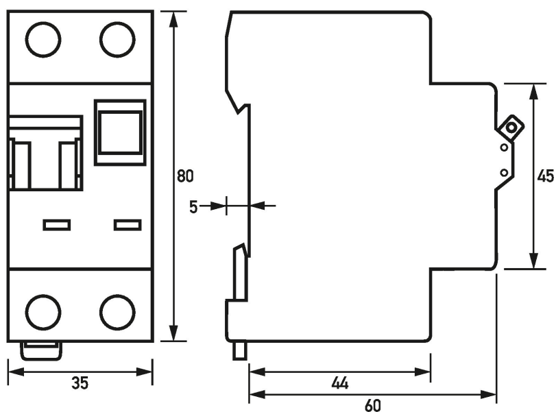
Dimensional drawing (Group view)
