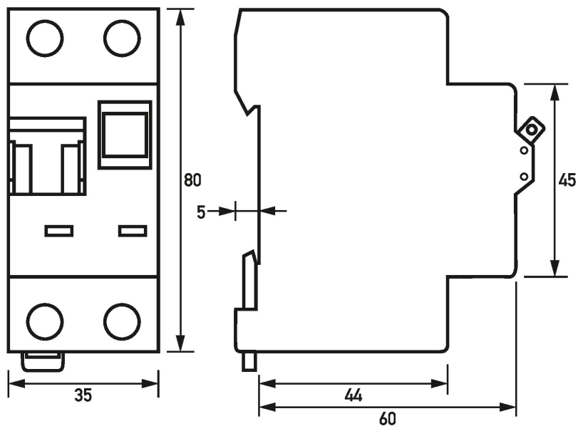
Dimensional drawing (Group view)
