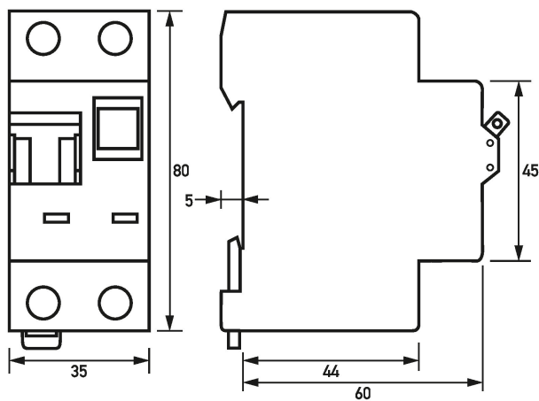
Dimensional drawing (Group view)
