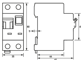
Dimensioned drawing residual current operated circuit-breakers with integral overcurrent protection DRCBO 3 Co4/0,30/1N-A
