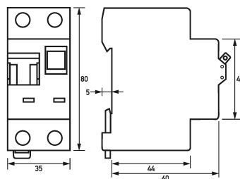
Dimensioned drawing residual current operated circuit-breakers with integral overcurrent protection DRCBO 3 B20/0,30/1N-A
