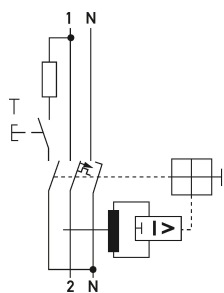
Wiring example residual current operated circuit-breakers with integral overcurrent protection DRCBO 3 B20/0,30/1N-A
