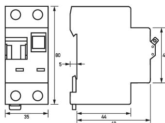
Dimensioned drawing residual current operated circuit-breakers with integral overcurrent protection DRCBO 3 B16/0,30/1N-A
