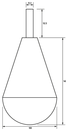
Dimensional drawing Group view
