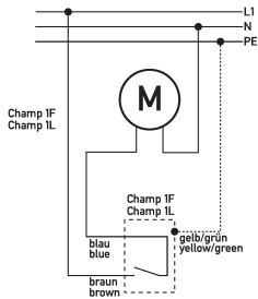
Wiring example float switches Champ 1 GS-L 03 m
