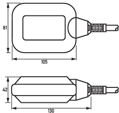
Dimensioned drawing float switches Champ 1 GS-L 03 m
