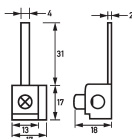
Dimensional drawing Group view
