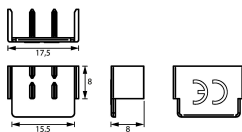
Dimensional drawing Group view
