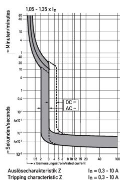
Diagrams miniature circuit-breakers DLS 6i Zo,8-3
