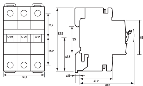
Dimensioned drawing miniature circuit-breakers DLS 6i Zo,8-3
