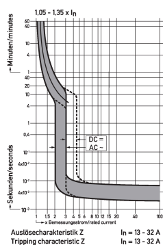
Diagrams miniature circuit-breakers DLS 6i Z20-2
