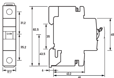
Dimensioned drawing miniature circuit-breakers DLS 6i Z02-1
