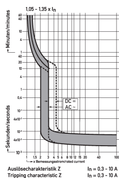
Diagrams miniature circuit-breakers DLS 6i Z02-1
