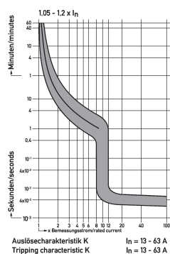
Diagrams miniature circuit-breakers DLS 6i K13-4
