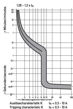
Diagrams miniature circuit-breakers DLS 6i K10-3
