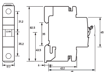
Dimensioned drawing miniature circuit-breakers DLS 6i, K-characteristic, 10 kA
