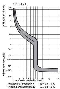
Diagrams miniature circuit-breakers DLS 6i, K-characteristic, 10 kA
