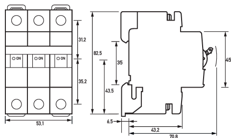
Dimensioned drawing miniature circuit-breakers DLS 6i D25-3
