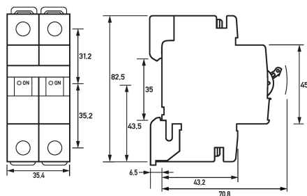
Dimensioned drawing miniature circuit-breakers DLS 6i D10-2
