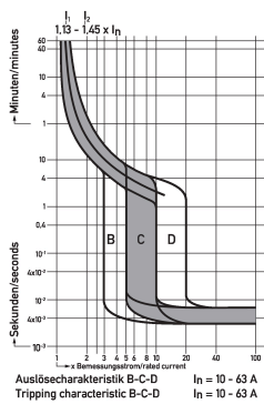
Diagrams miniature circuit-breakers DLS 6i, D-characteristic, 10 kA
