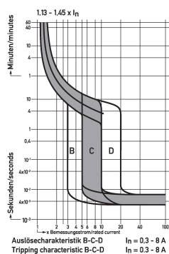
Diagrams miniature circuit-breakers DLS 6i Co2-1+N
