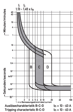
Diagrams miniature circuit-breakers DLS 6i, C-characteristic, 10 kA
