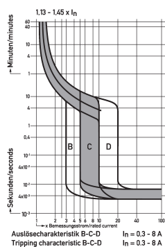
Diagrams miniature circuit-breakers DLS 6i Bo6-3
