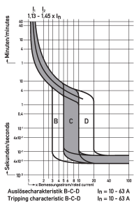
Characteristic Char. B, C, D
