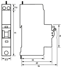
Dimensional drawing Group view
