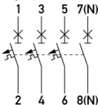
Wiring diagram
