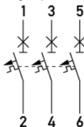
Wiring diagram
