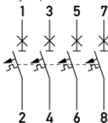
Wiring diagram
