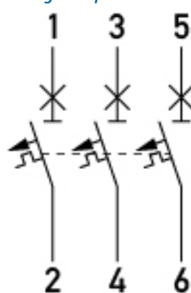
Wiring diagram
