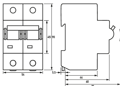
Dimensioned drawing miniature circuit-breakers DMCB 2 C125-2
