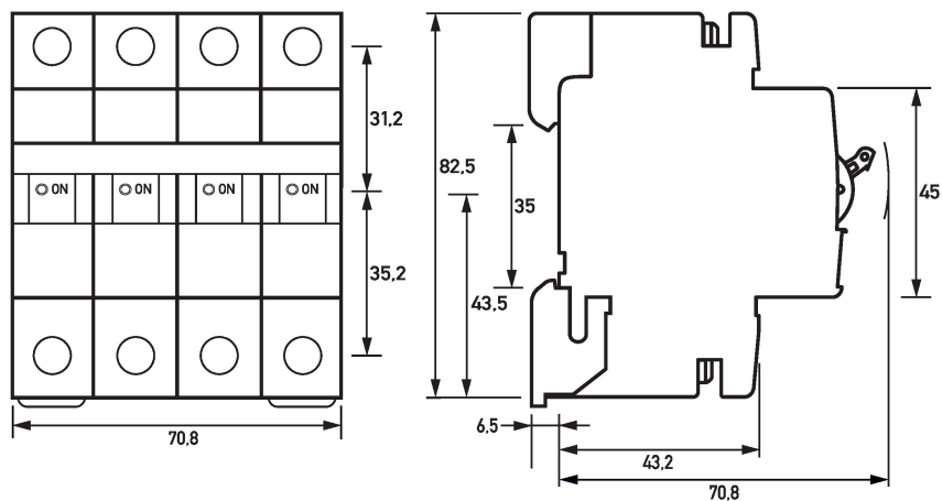
Dimensional drawing DLS 6h, C-characteristic, four-pole (Group view)
