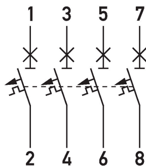
Wiring diagram DLS 6h, C-characteristic, four-pole
