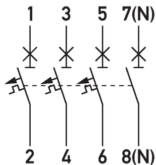
Wiring diagram DLS 6h, C-characteristic, three-pole+N
