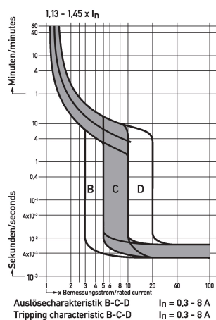
Characteristic Char. B, C, D
